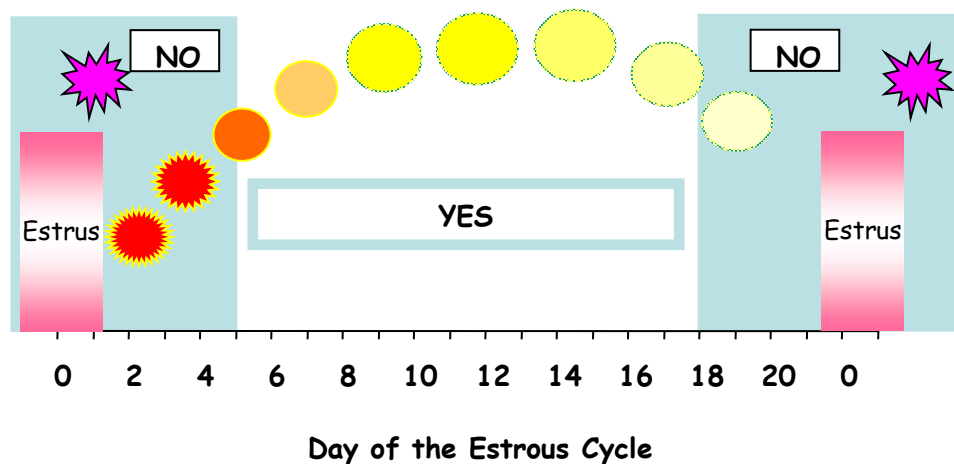
Figure 7. Effect of stage of the bovine estrous cycle on luteal responsiveness to \text{PGF}_{2\alpha} . Bovine corpora lutea will not respond to an injection of \text{PGF}_{2\alpha} during the first five days of the cycle. Therefore, \text{PGF}_{2\alpha} should not be injected at the beginning of progestin treatment (Modified from Kojima and Patterson, 2003).
